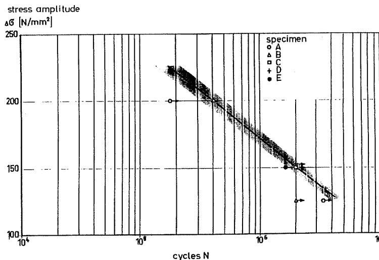
Fig. 7. \Delta\sigma -N-curve (WÖHLER-diagram) for preloaded cables on the base of 25 % wire crackes
