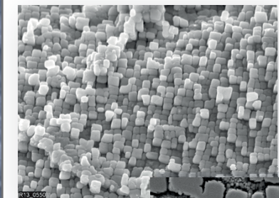
Gamma-prime phase in a cast nickel alloy (SEM image of the fracture surface)
