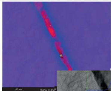
TEM: element mapping across a grain boundary
