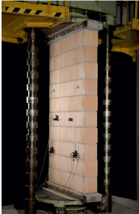
Determination of compressive strength and deformation behavior of masonry
